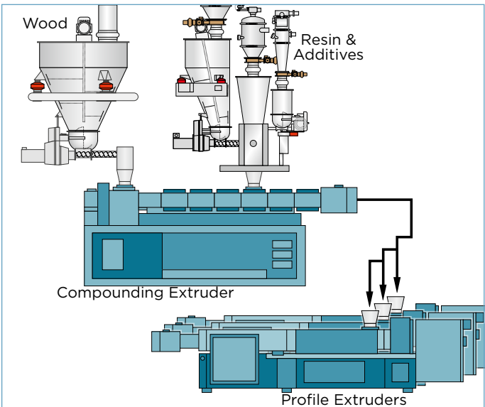
4. A high-speed compounding extruder supplies multiple single or twin screw profiling extruders. Alternatively, compounding extruder feeds a gear pump to produce the profile.
