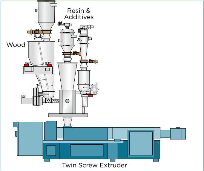
1. Pre-dried wood along with resin/regrinds and additives all enter at the throat of a twin screw pelletizing extruder.
